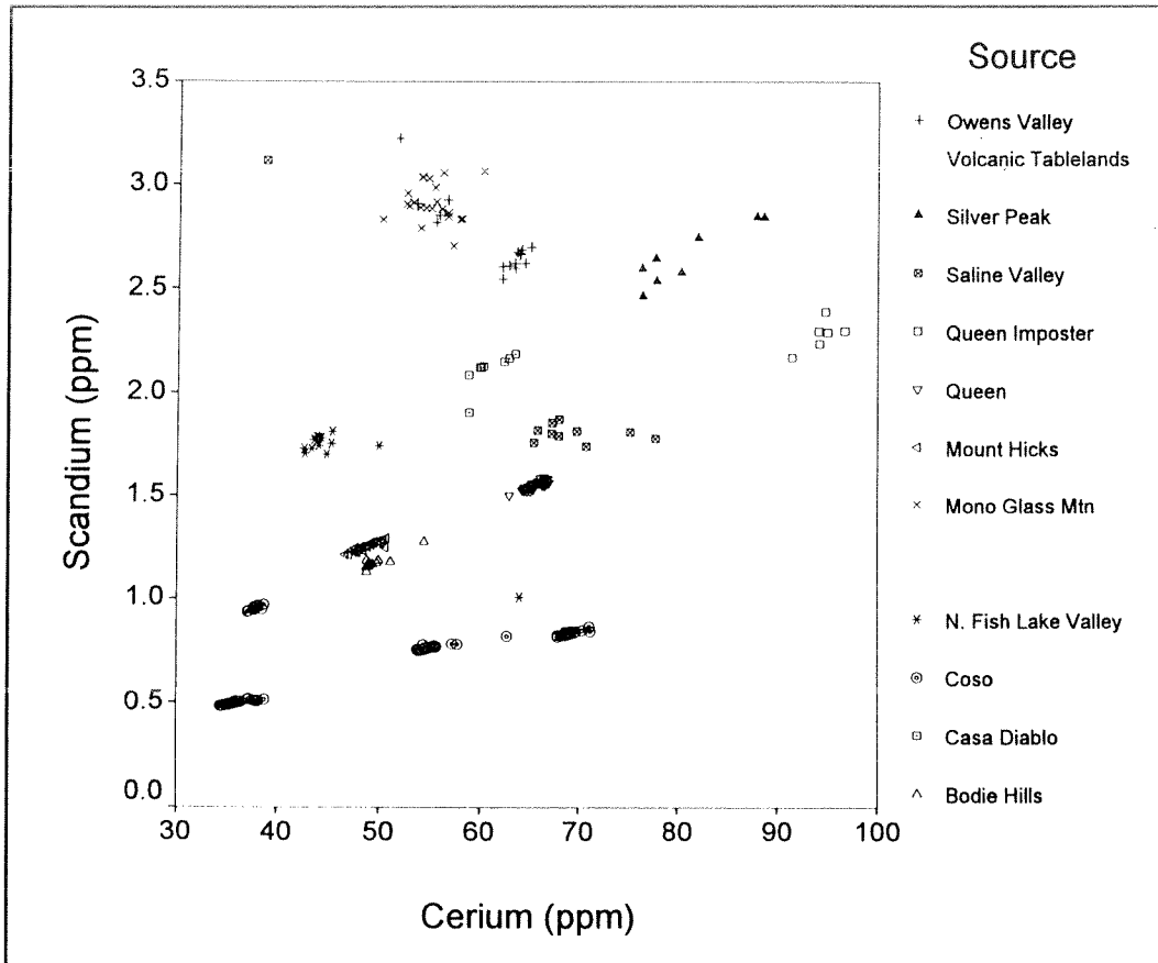
Fig. 3. Bivariate plot of scandium and cerium for major obsidian sources in the study region.
