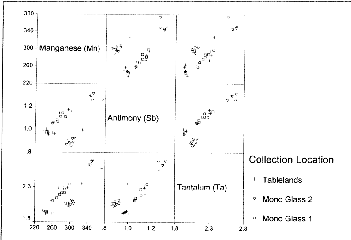
Fig. 5. Bivariate plots of manganese, antimony, and tantalum for Owens Valley Volcanic Tablelands and Mono Glass Mountain obsidian nodules. All values are in ppm.
