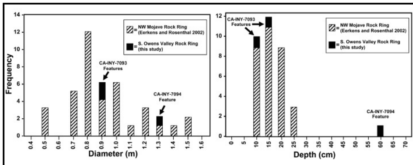
Figure 4. Comparison of diameter and depth of Owens Valley versus NW Mojave features.
