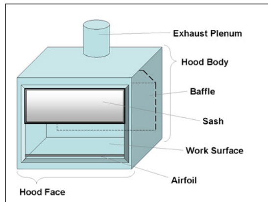
Figure IV-II. Fume Hood
