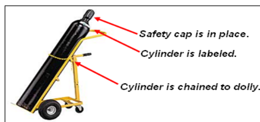
Figure VI-IV. Correct Cylinder Transport
